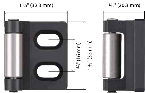
P/N. DXAS203 Top Strike For DX2PV, DX2PW.
