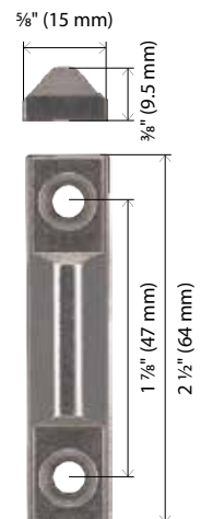
P/N. DXAS224* Bottom Strike Optional for DX2PV and DX2PW. (Grade 2)
