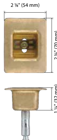
P/N. DXAS227/227F Bottom Strike Standard for DX2PV/FV, DX2PC/FC, DX2PW/FW.
