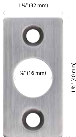
P/N. DXAS225* Bottom Strike For DX2PV, DX2PC, DX2PW with round slide bolt. (Grade 2)
