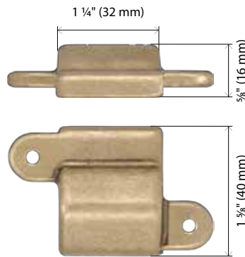
P/N. DXAS216 Top Strike Standard for DX2PC/FC.
