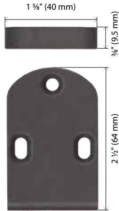
P/N. DXAS215* Top Strike For flush transom DX2PV/FV, DX2PW/FW.
